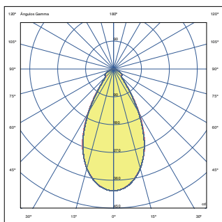
Optic lens 60°
