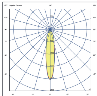
Optic lens 30°
