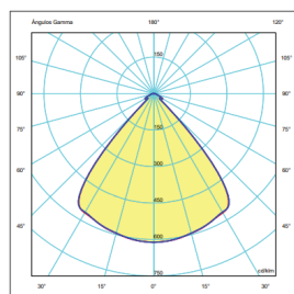
Acrylic lens, metal shade up
