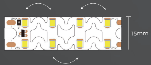
Bending angle: 0^\circ < \theta < 10^\circ Horizontal bending: D_{min} > 320mm
