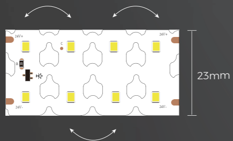
Horizontal bending: D_{min} \geq 1000mm
